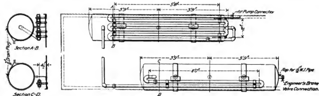
Figs. 2677-2680. Location and Arrangement of Main Reservoir, Atlantic (4-4-2) Locomotive, Pennsylvania R. R.
